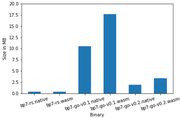
Fig. 7. Binary sizes of the various benchmarks
